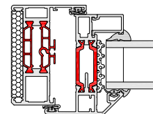
► 58BW ST HI MULLION / TRANSOM
