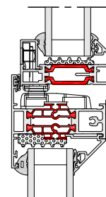
► 58BW ST HI MULLION / TRANSOM
